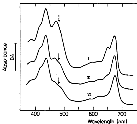
Fig.2. Room temperature absorbance spectra of chl-protein complexes extracted from gel bands I, III and VII of fig.1. Arrows indicate A_{450} (compare fig.1).
